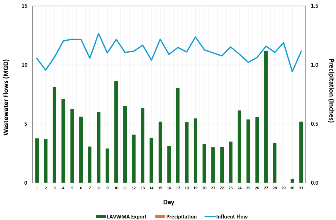
Figure 3. Wastewater Flows and Precipitation
