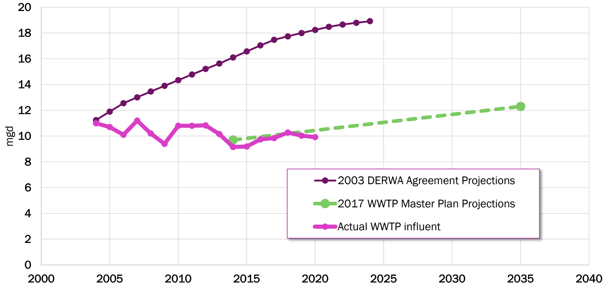
WWTP Influent – Average Dry Weather Flow
